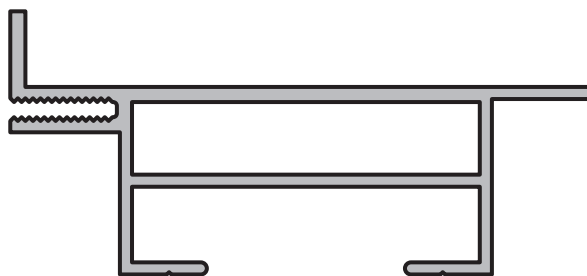
PREMARCO UNIVERSAL
